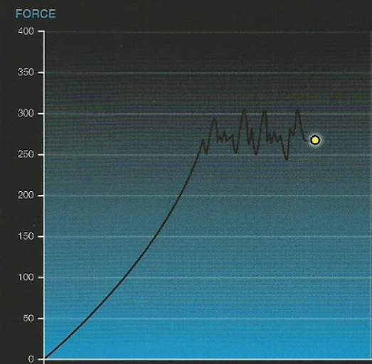
TEAR STRENGTH WEFT
