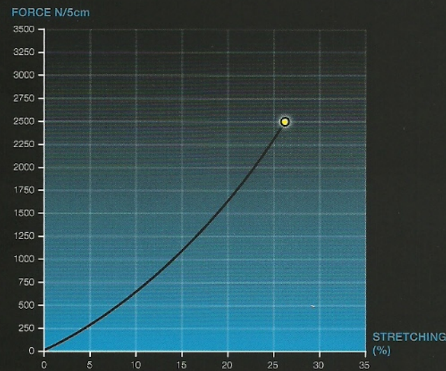
BREAKING STRENGTH WARP
